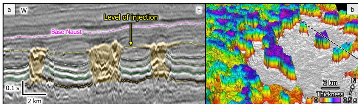
Fig. 5. Sand injectites within the Neogene sediment packages. a) Seismic expression of three isolated injectite mounds with internal chaotic seismic facies (yellow). b) Isopach map blended over structure map showing geomorphology and thickness of the injectites. Seismic data courtesy: TGS.
